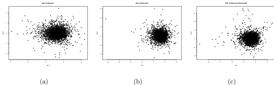
Figure 4.13: Plot of three different 2 dimensional data set. (a) is training data, (b) is testing data and (c) is fitted data. All of these three data sets have the sample size is 5000. In figures, xlab represents the first component and ylab represents the second component.
