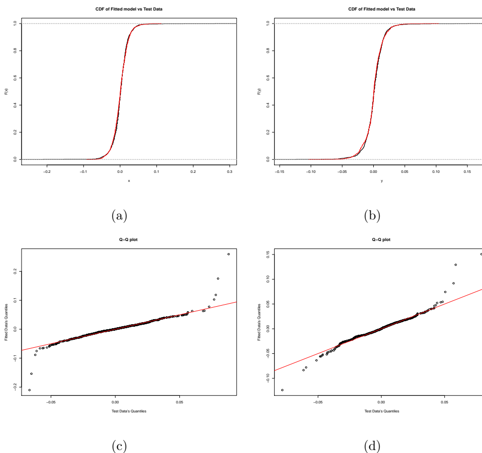
Figure 5.8: TS CDF plots for the (a) FB and (b) GOOGL data, red line represents CDF of fitted data, and black line represents CDF of the testing data. Figure(c) and (d) are the fitted TS qq-plots for the (a) FB and (b) GOOGL data. These compare the quantiles of the testing data with the fitted data. The diagonal (red) line is the line y = x .
