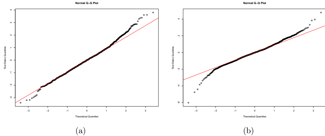
Figure 4.19: Normal qq-plots for the testing data. The plot in a) is for the first component (CAD/USD) and the plot in b) is for the second component (EUR/USD). The diagonal (red) line is the line passing through the first and third quartiles.
