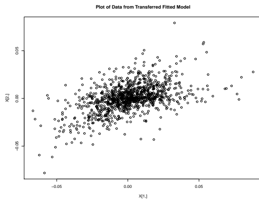
Figure 5.7: The same sample size 1258. In figures, x-axis represents the first component FB and y-axis represents the second component GOOGL.
