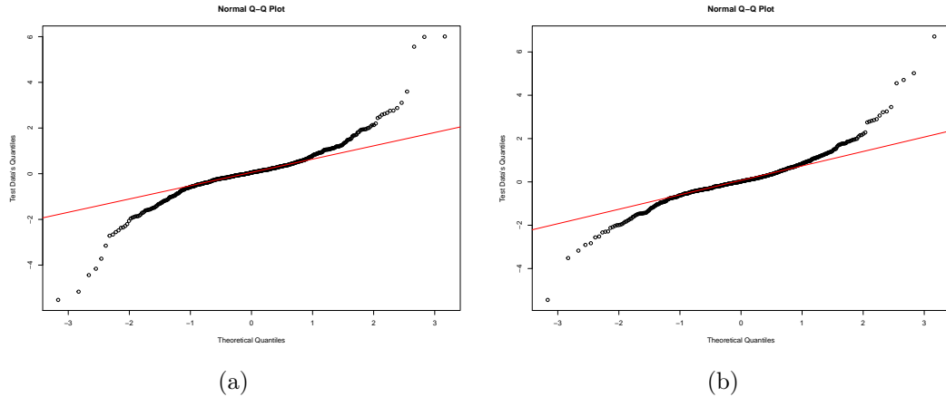
Figure 4.30: Normal qq-plots for the testing data. The plot in a) is for the first component (BTC/USD) and the plot in b) is for the second component (ETH/USD). The diagonal (red) line is the line passing through the first and third quartiles.
