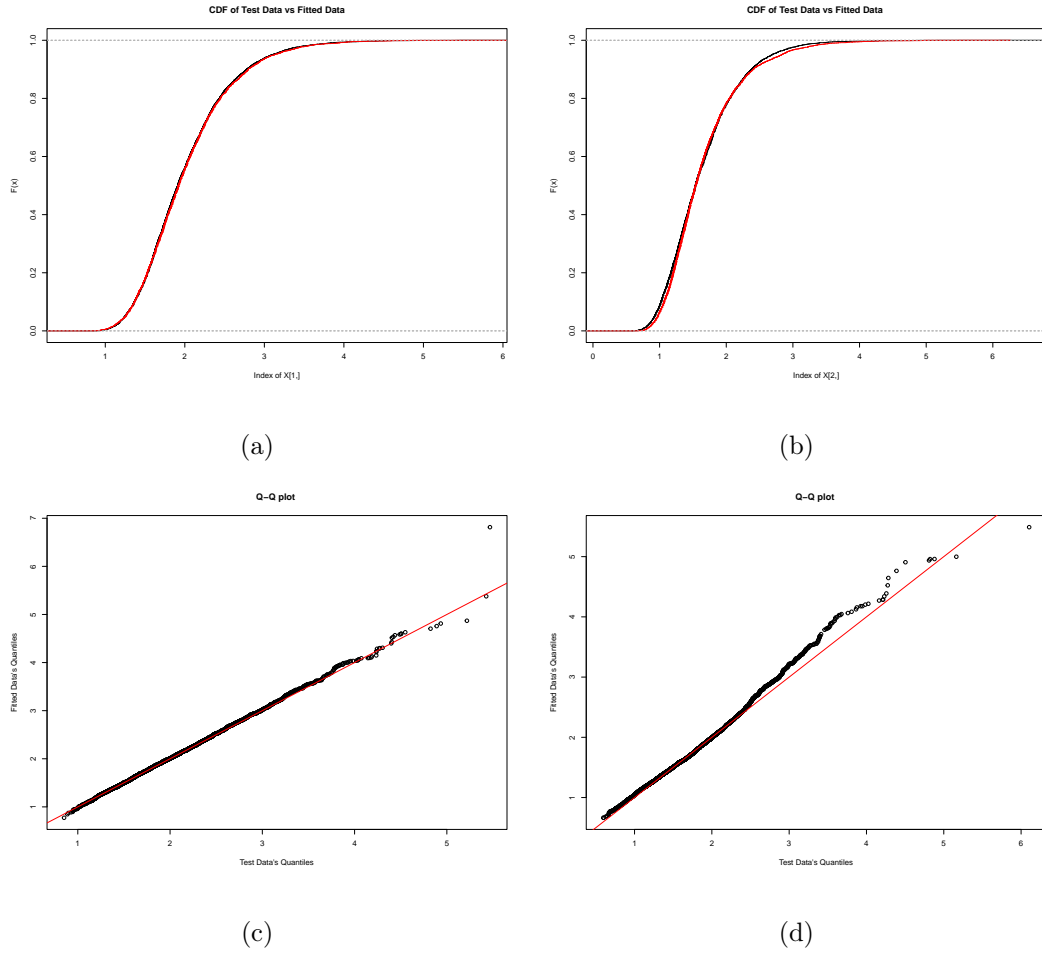
Figure 4.11: Figure(a) is CDF plots between fitted data and testing data in the first component. Figure(b) is CDF plots in the second component. The red line represents fitted data, and black line represents testing data. Figure(c) is a qq-plot of testing data and fitted data in the first component and Figure(d) is in the second component. In these two plots, xlab is quantiles of test data and ylab is quantiles of fitted data, also red line is y = x .
