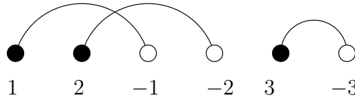
FIGURE 2. The arc diagram associated to (1, 2, -1, -2, 3, -3)
